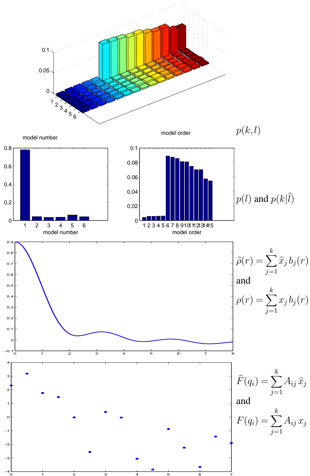
Fig. 2: a) p(k, l|\mathbf{y}) , p(l|\mathbf{y}) and p(k|\mathbf{y}, \hat{l}) , b) original \rho(r) and estimated \hat{\rho}(r) , c) original F(q_i) and estimated \hat{F}(q_i) .
